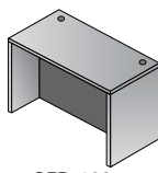
OFD-103 60"x30"x29" Desk Shell List $305
